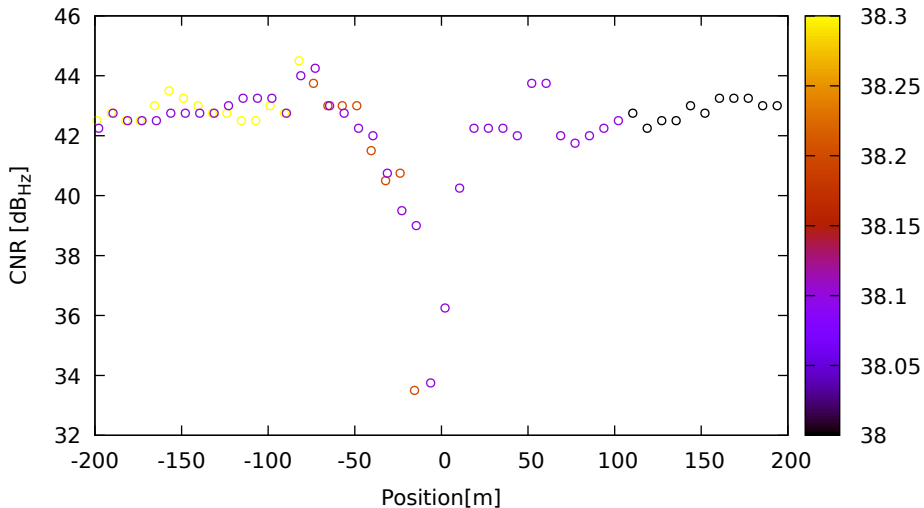
CNR vs position for C09 (B3) on LeicaGS18 - DOY 263 jam. 1
