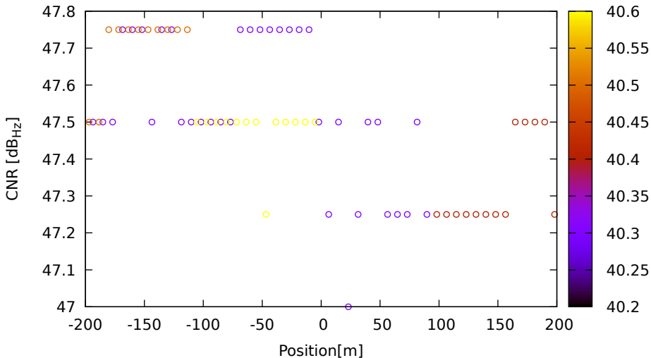
CNR vs position for C28 (B3) on LeicaGS18 - DOY 263 jam. 3
