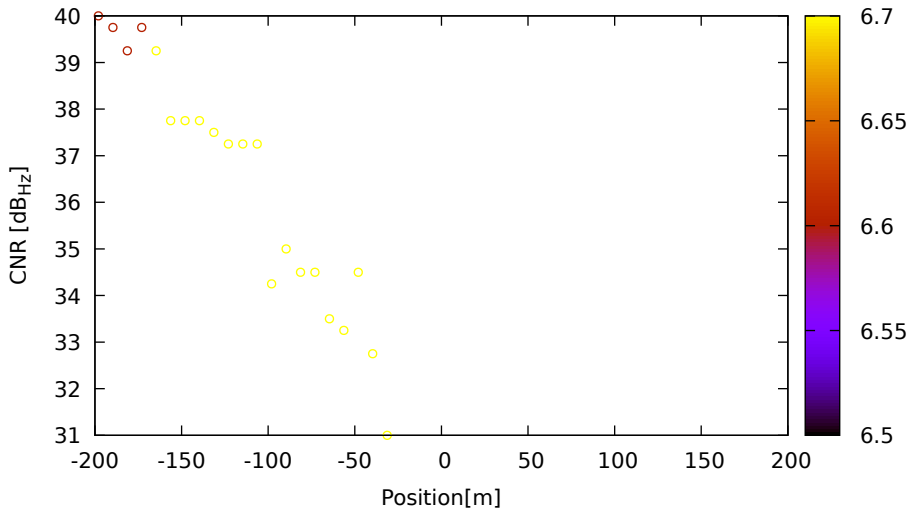
CNR vs position for E09 (E1) on LeicaGS18 - DOY 263 jam. 2
