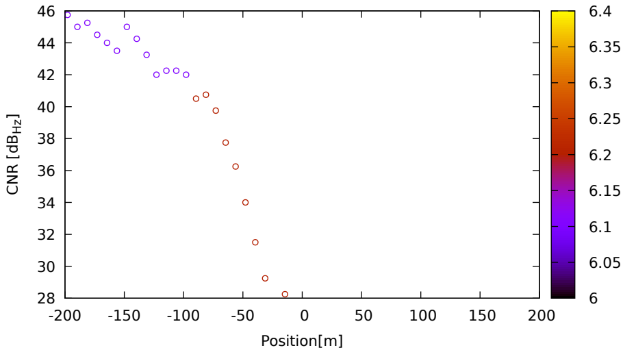
CNR vs position for E09 (E5) on LeicaGS18 - DOY 263 jam. 1
