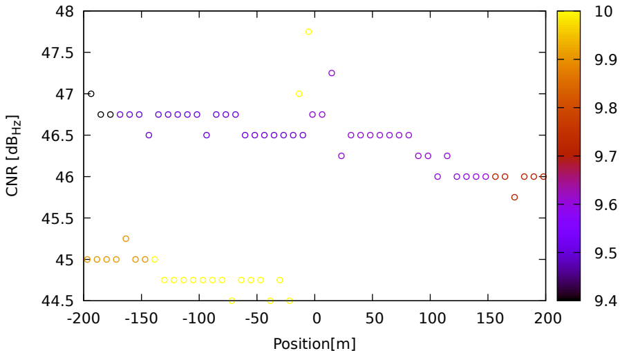
CNR vs position for E09 (E5) on LeicaGS18 - DOY 263 jam. 3
