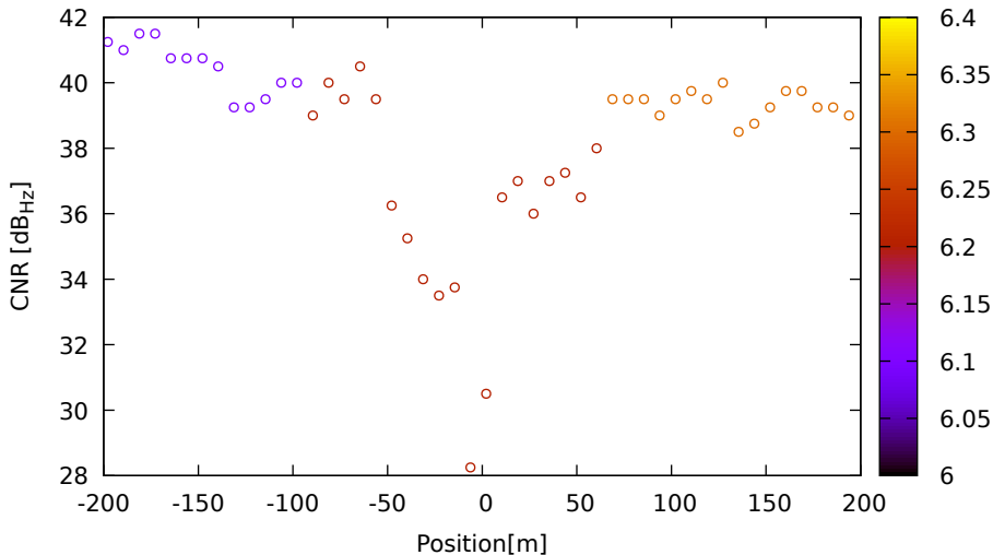
CNR vs position for E09 (E5a) on LeicaGS18 - DOY 263 jam. 1
