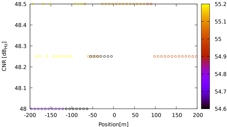
CNR vs position for E19 (E5b) on LeicaGS18 - DOY 263 jam. 3
