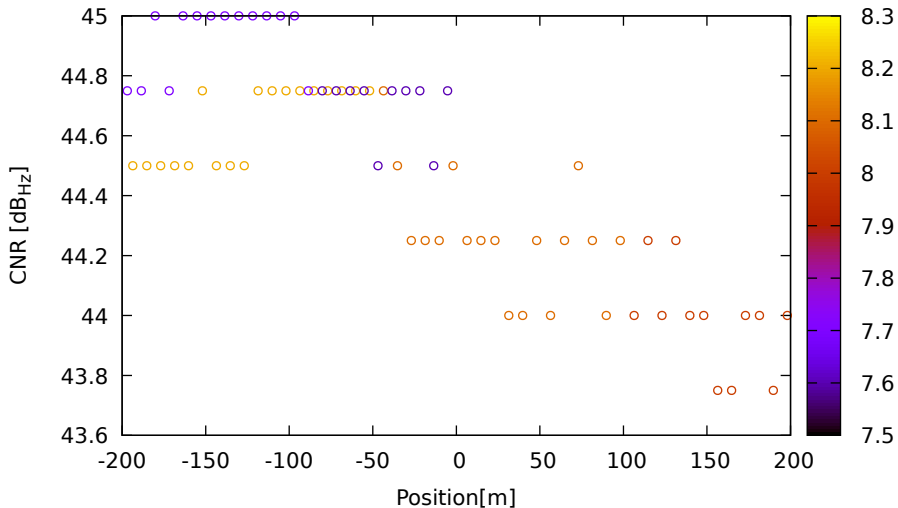
CNR vs position for E33 (E5) on LeicaGS18 - DOY 263 jam. 3
