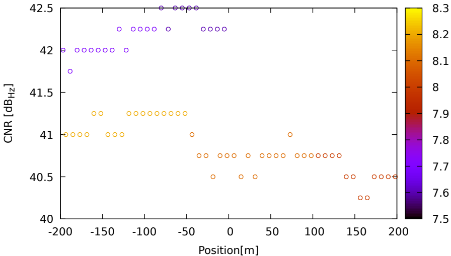
CNR vs position for E33 (E5a) on LeicaGS18 - DOY 263 jam. 3
