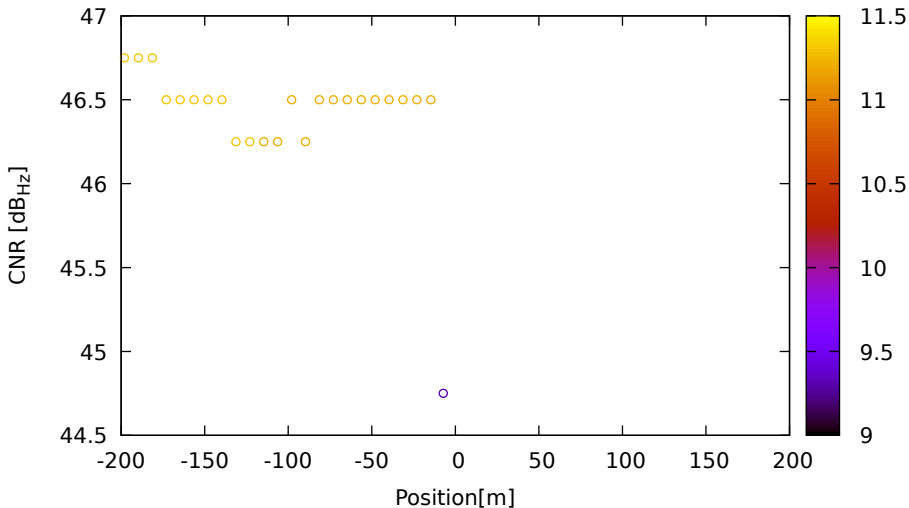
CNR vs position for E33 (E5b) on LeicaGS18 - DOY 263 jam. 2
