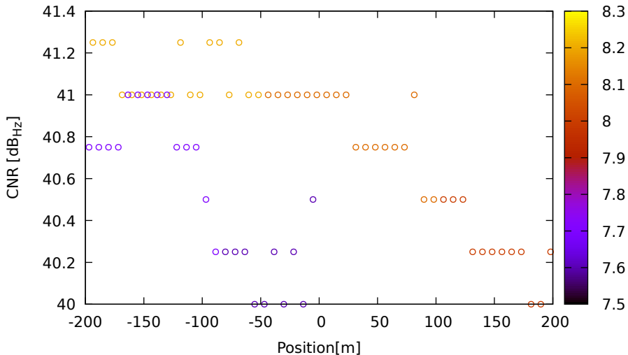
CNR vs position for E33 (E5b) on LeicaGS18 - DOY 263 jam. 3
