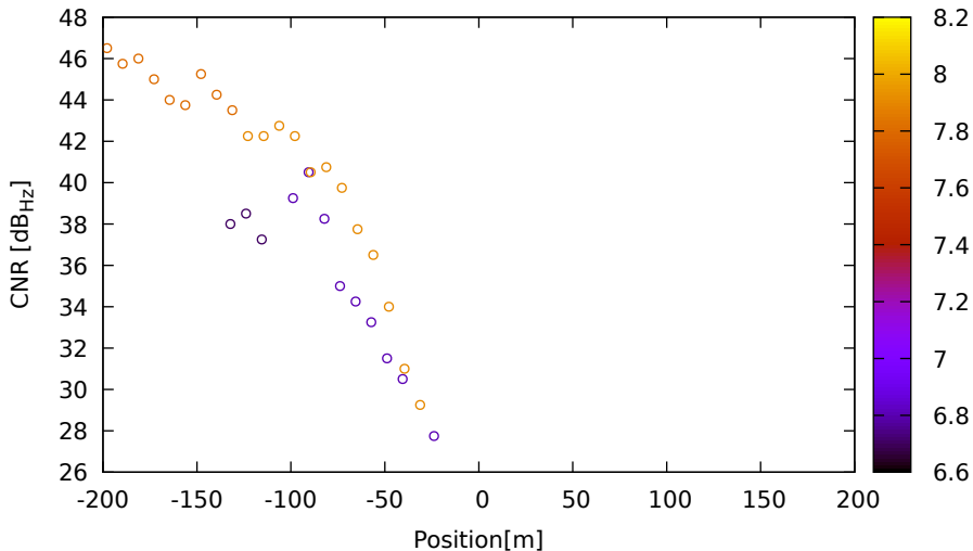
CNR vs position for E36 (E5) on LeicaGS18 - DOY 263 jam. 1
