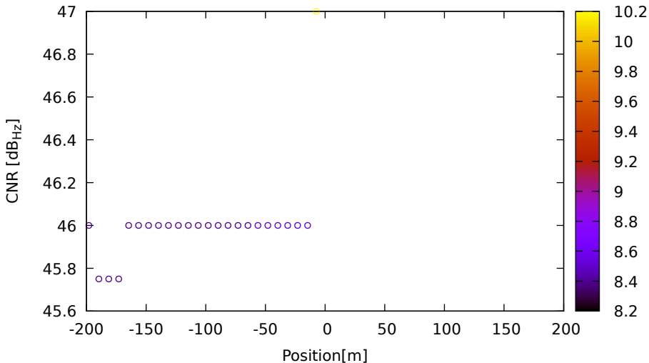
CNR vs position for E36 (E5) on LeicaGS18 - DOY 263 jam. 2
