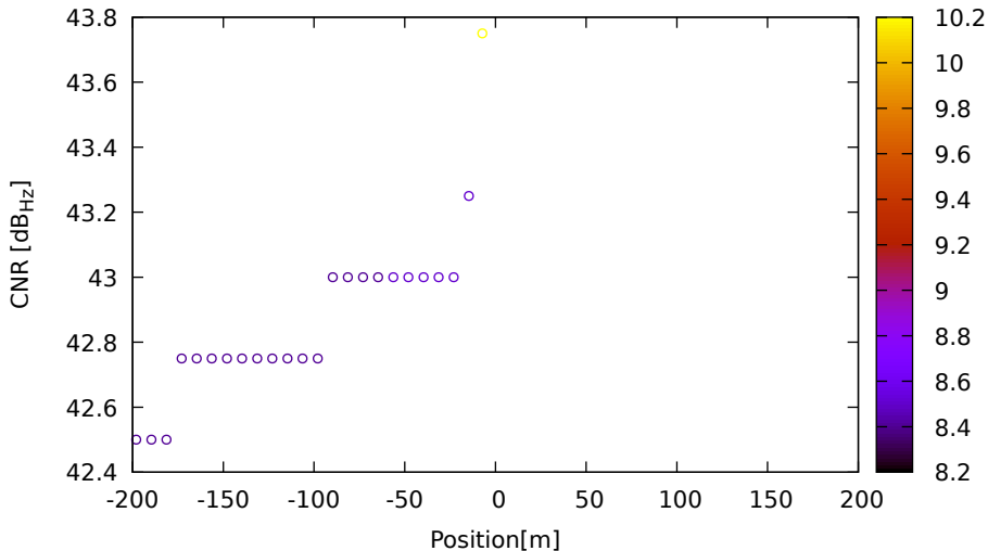
CNR vs position for E36 (E5a) on LeicaGS18 - DOY 263 jam. 2
