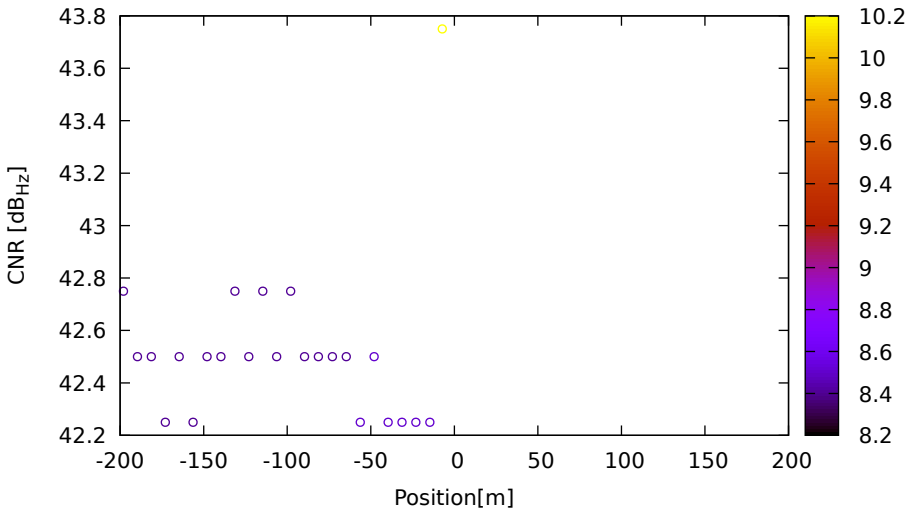
CNR vs position for E36 (E5b) on LeicaGS18 - DOY 263 jam. 2
