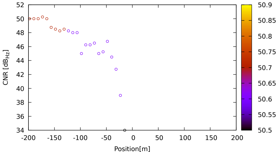
CNR vs position for G01 (L2) on LeicaGS18 - DOY 263 jam. 2
