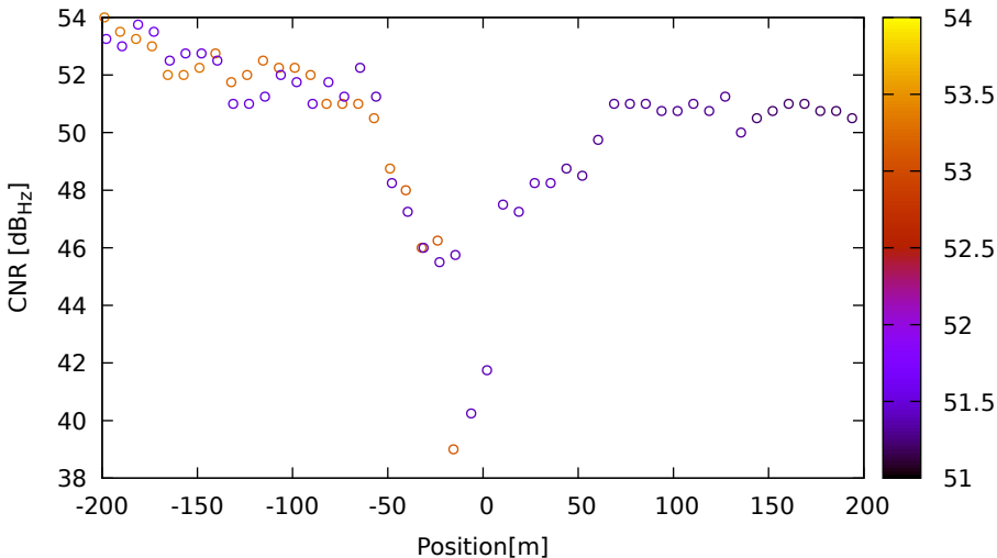
CNR vs position for G01 (L5) on LeicaGS18 - DOY 263 jam. 1
