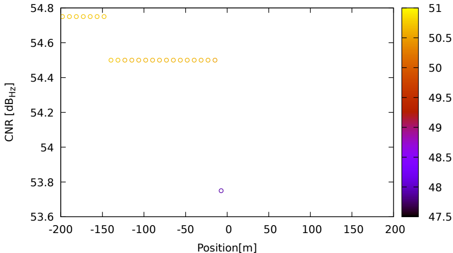
CNR vs position for G01 (L5) on LeicaGS18 - DOY 263 jam. 2
