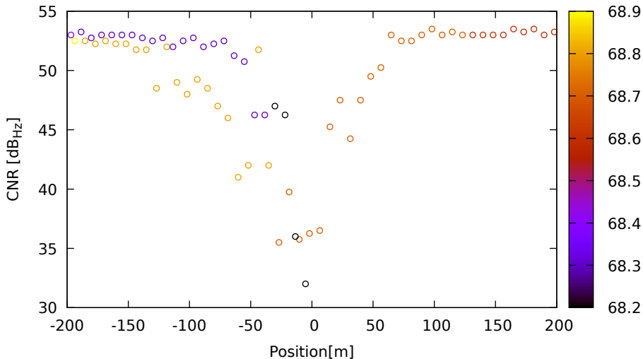
CNR vs position for G03 (L2) on LeicaGS18 - DOY 263 jam. 3
