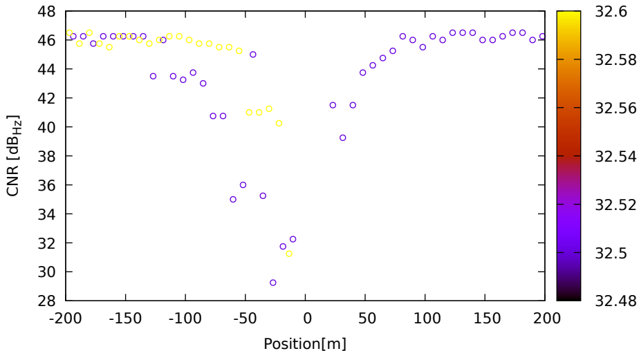
CNR vs position for G19 (L2) on LeicaGS18 - DOY 263 jam. 3
