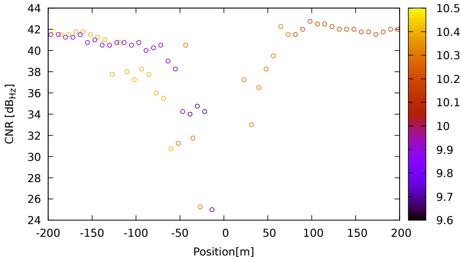
CNR vs position for G22 (L1) on LeicaGS18 - DOY 263 jam. 3
