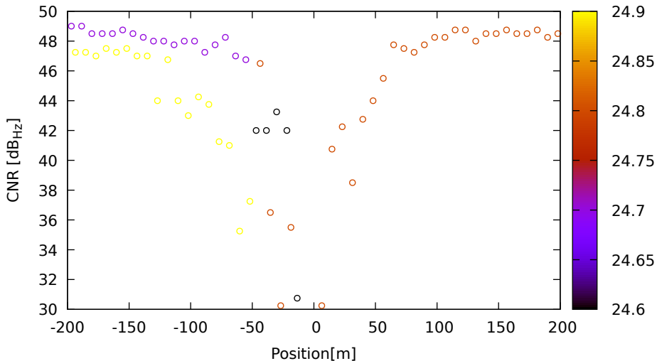
CNR vs position for G31 (L2) on LeicaGS18 - DOY 263 jam. 3
