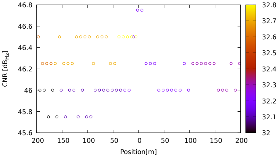
CNR vs position for R03 (G2) on LeicaGS18 - DOY 263 jam. 3
