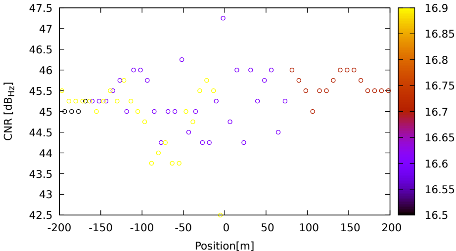
CNR vs position for R11 (G1) on LeicaGS18 - DOY 263 jam. 3
