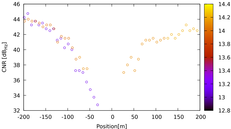
CNR vs position for R11 (G2) on LeicaGS18 - DOY 263 jam. 1
