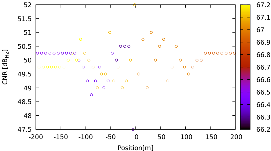
CNR vs position for R17 (G1) on LeicaGS18 - DOY 263 jam. 3
