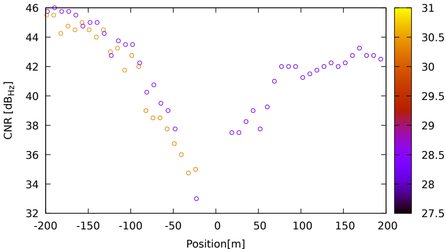
CNR vs position for R24 (G2) on LeicaGS18 - DOY 263 jam. 1
