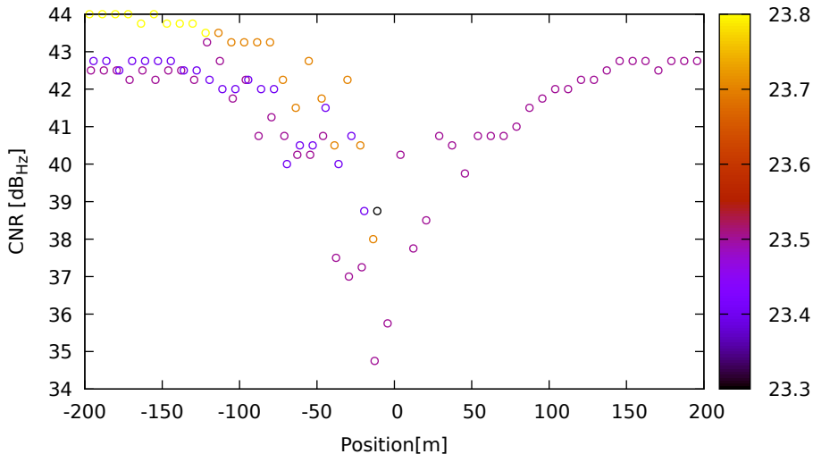
CNR vs position for C06 (B1) on LeicaGS18 - DOY 263 jam. 3
