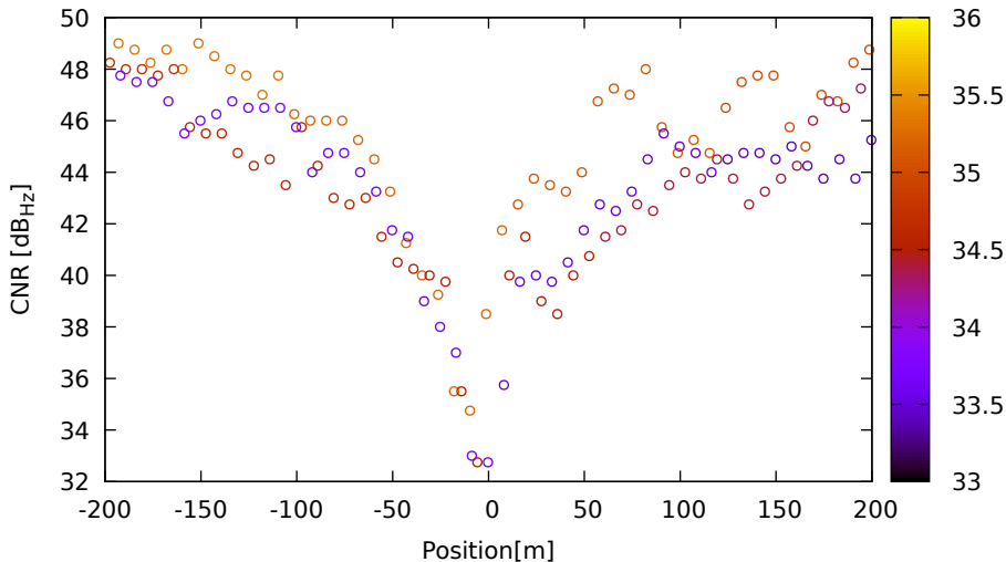
CNR vs position for C11 (B2) on LeicaGS18 - DOY 263 jam. 1
