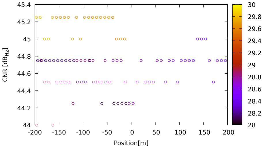
CNR vs position for C11 (B3) on LeicaGS18 - DOY 263 jam. 3
