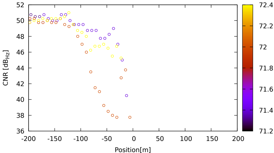
CNR vs position for C14 (B1) on LeicaGS18 - DOY 263 jam. 2
