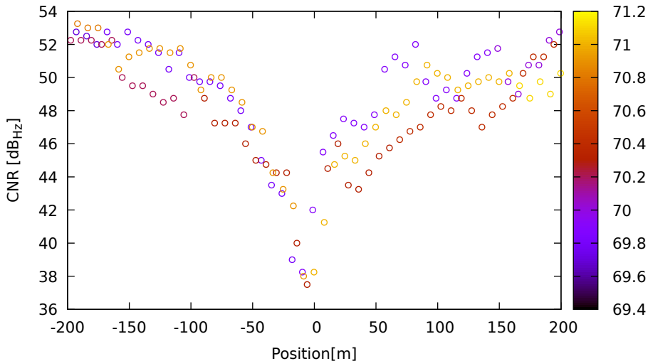
CNR vs position for C14 (B2) on LeicaGS18 - DOY 263 jam. 1
