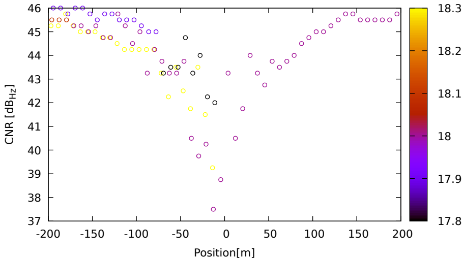
CNR vs position for C16 (B1) on LeicaGS18 - DOY 263 jam. 3
