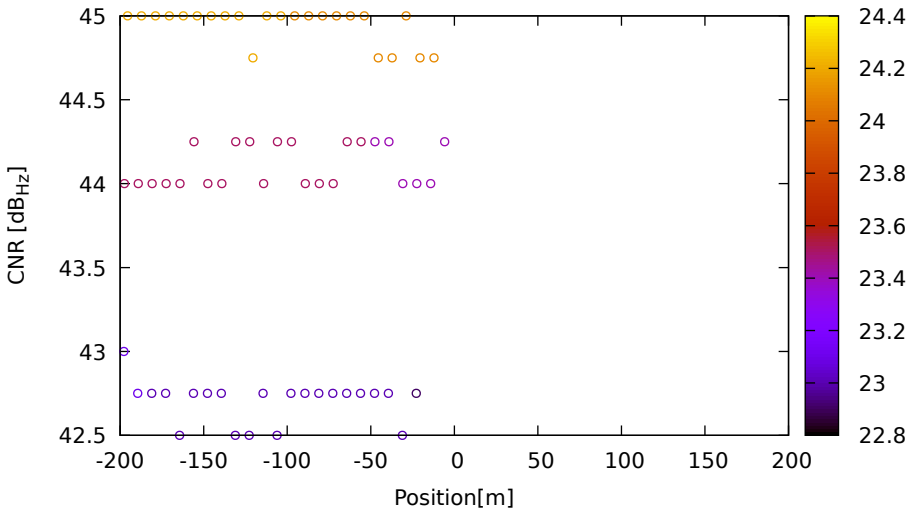
CNR vs position for C21 (B3) on LeicaGS18 - DOY 263 jam. 2
