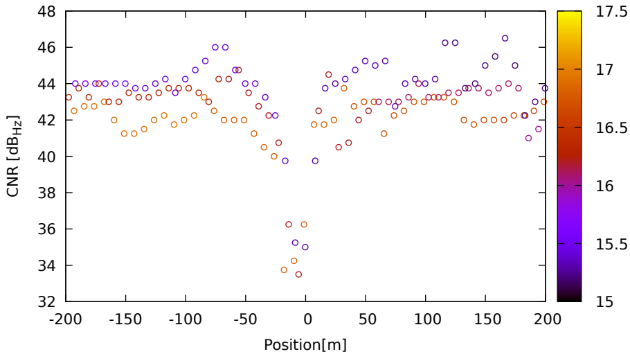
CNR vs position for C34 (B3) on LeicaGS18 - DOY 263 jam. 1
