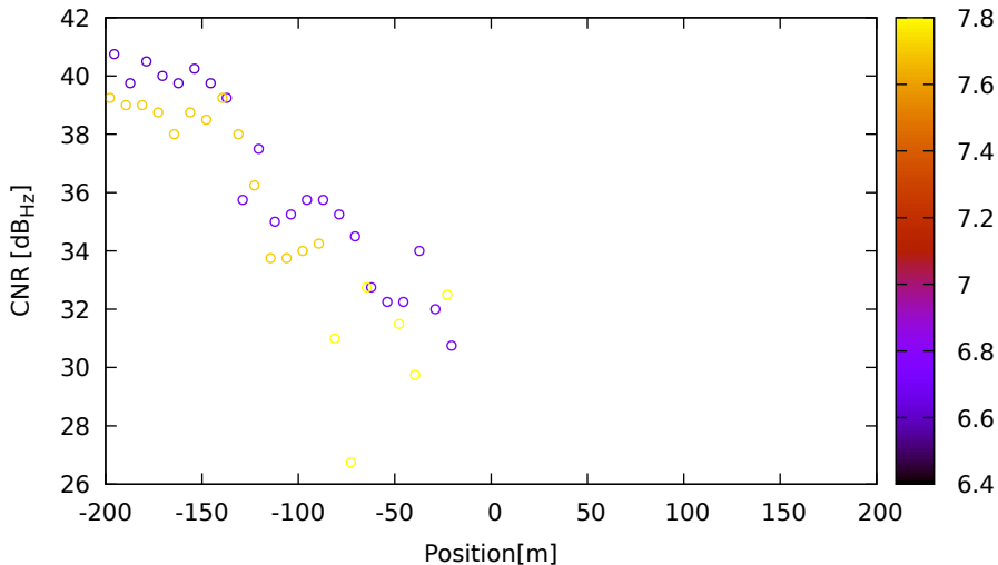
CNR vs position for E09 (E1) on LeicaGS18 - DOY 263 jam. 2
