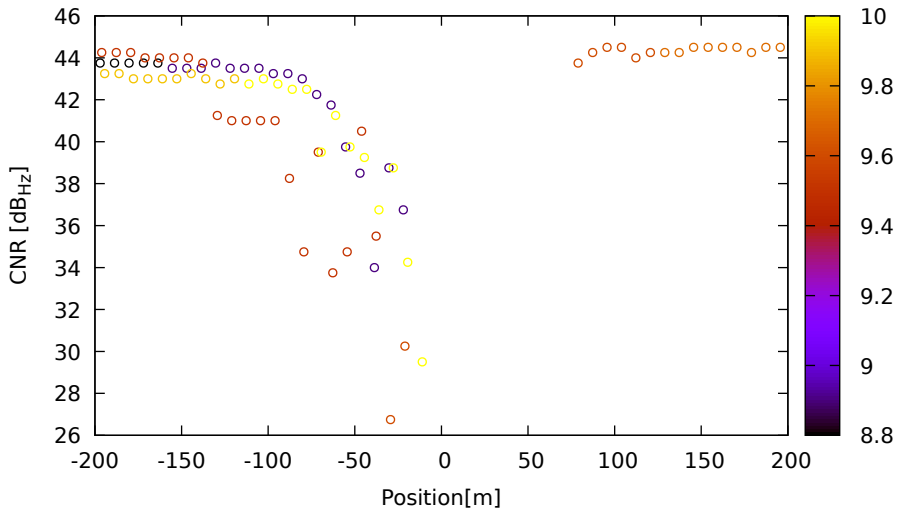
CNR vs position for E09 (E1) on LeicaGS18 - DOY 263 jam. 3
