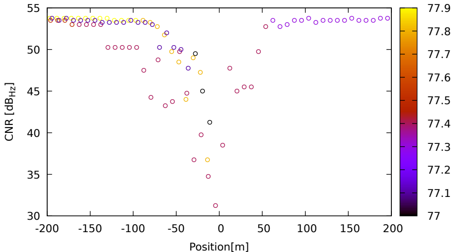
CNR vs position for E10 (E1) on LeicaGS18 - DOY 263 jam. 3
