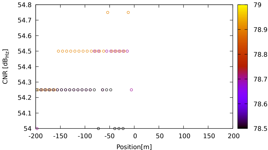
CNR vs position for E10 (E5a) on LeicaGS18 - DOY 263 jam. 2
