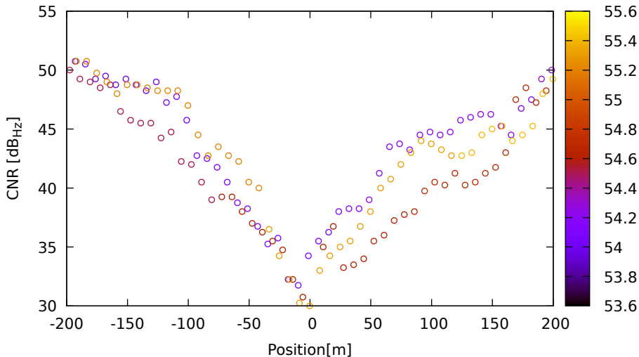
CNR vs position for E11 (E5) on LeicaGS18 - DOY 263 jam. 1
