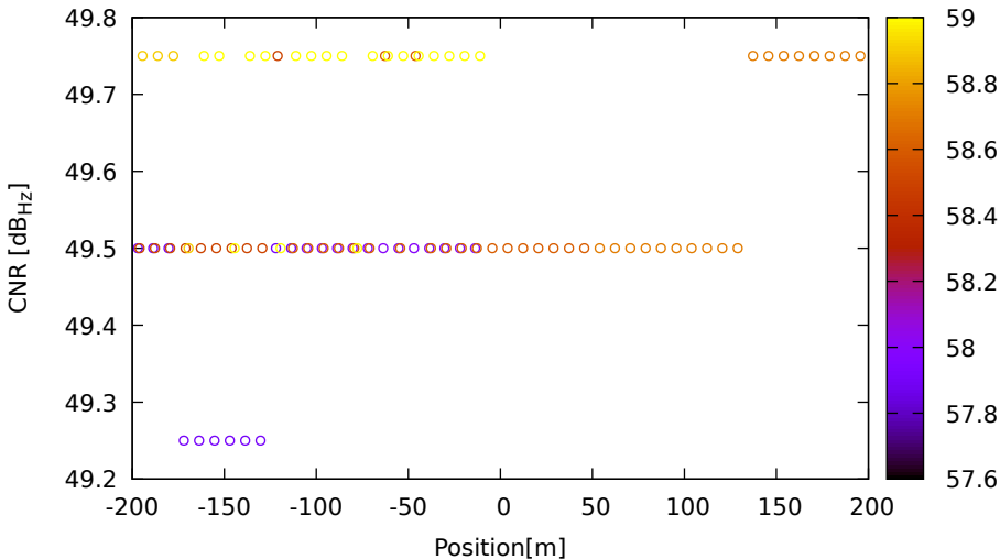
CNR vs position for E11 (E5b) on LeicaGS18 - DOY 263 jam. 3
