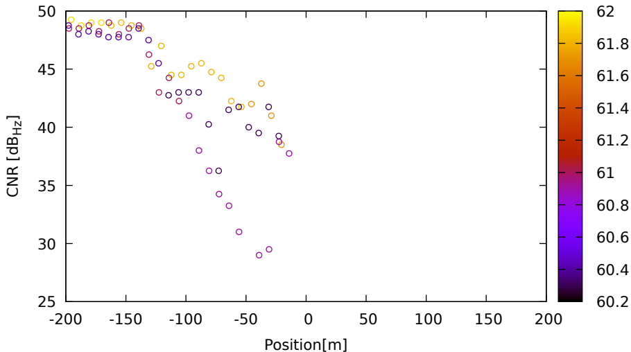
CNR vs position for E12 (E1) on LeicaGS18 - DOY 263 jam. 2
