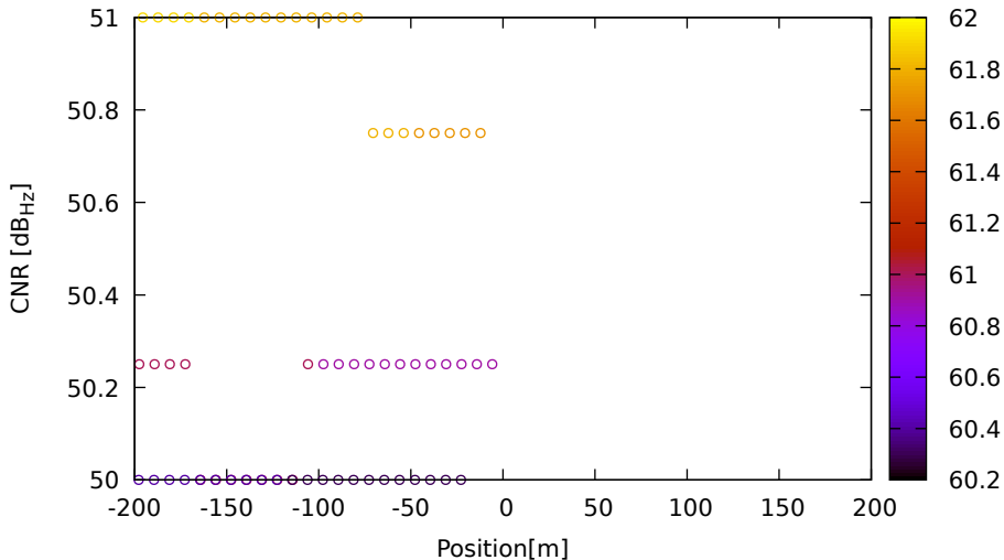
CNR vs position for E12 (E5b) on LeicaGS18 - DOY 263 jam. 2
