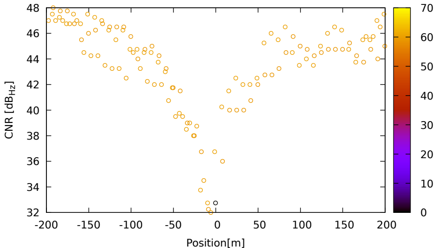
CNR vs position for E19 (E5b) on LeicaGS18 - DOY 263 jam. 1
