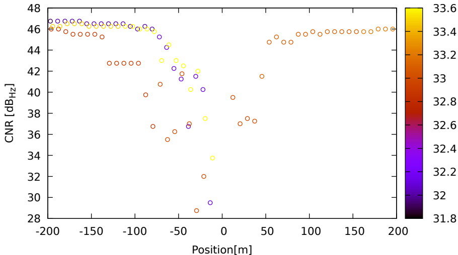
CNR vs position for G09 (L1) on LeicaGS18 - DOY 263 jam. 3
