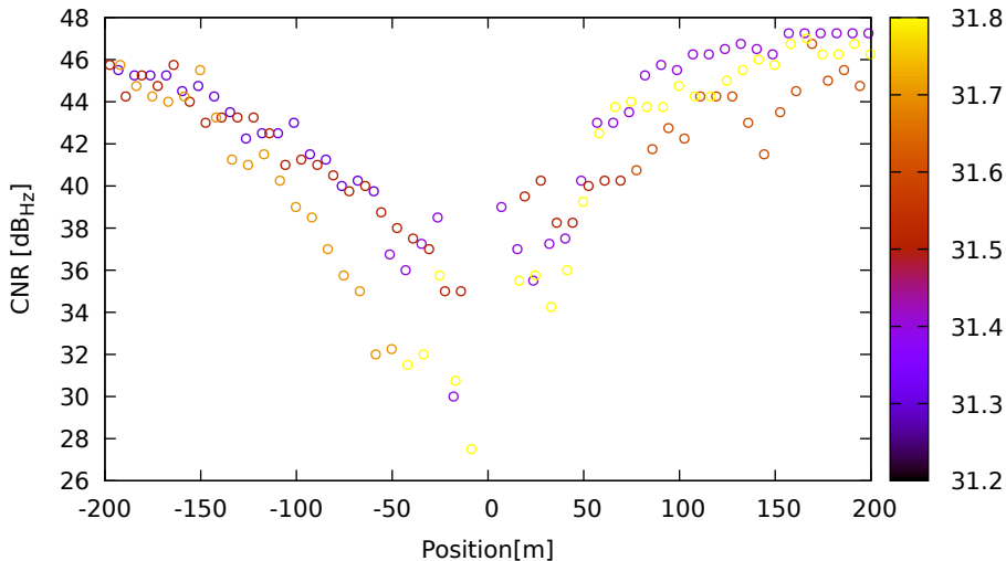
CNR vs position for G19 (L1) on LeicaGS18 - DOY 263 jam. 1
