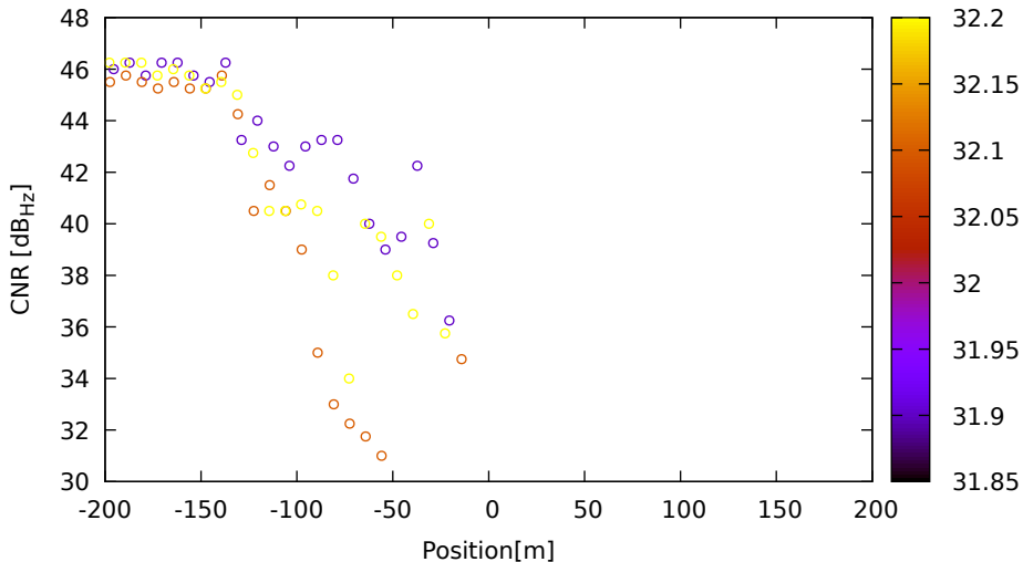
CNR vs position for G19 (L2) on LeicaGS18 - DOY 263 jam. 2
