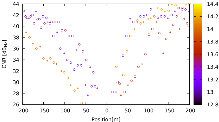
CNR vs position for R11 (G1) on LeicaGS18 - DOY 263 jam. 1
