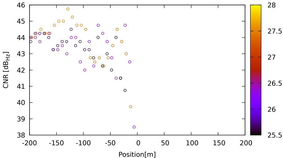
CNR vs position for R24 (G1) on LeicaGS18 - DOY 263 jam. 2
