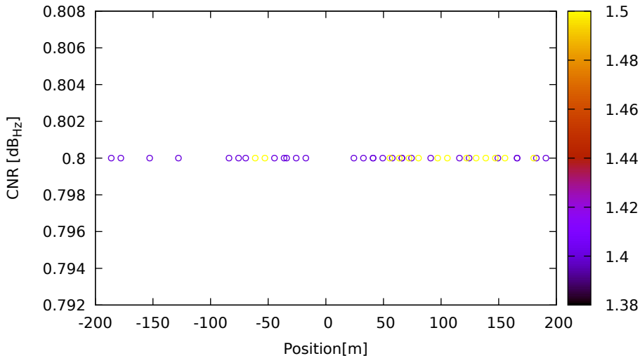
CNR vs position for 28 (G1) on SamsungS20 - DOY 263 jam. 2
